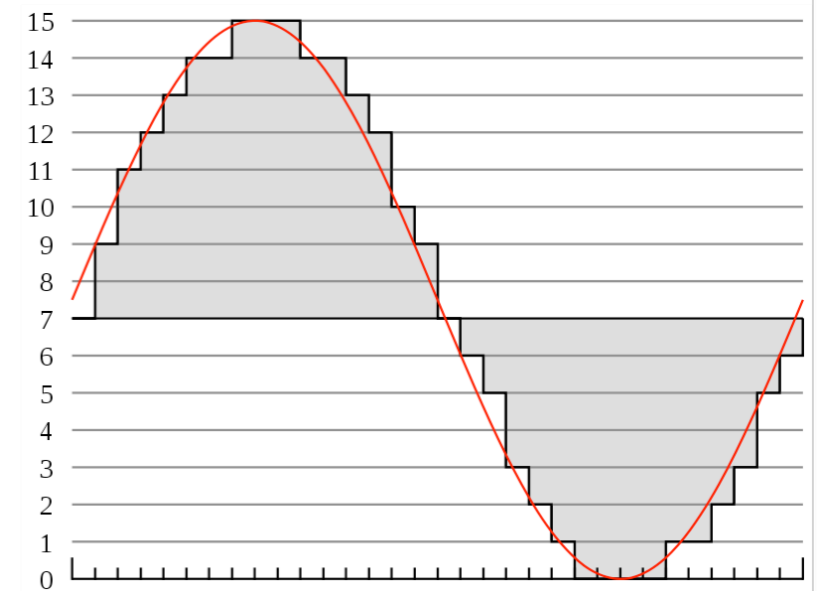
Sampling and quantization of a signal (red) for 4-bit PCM
